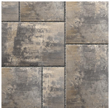
LARGE RECTANGLE 233mm x 349.5mm x 60mm 9 1/4" x 13 3/4" x 2 3/8"
