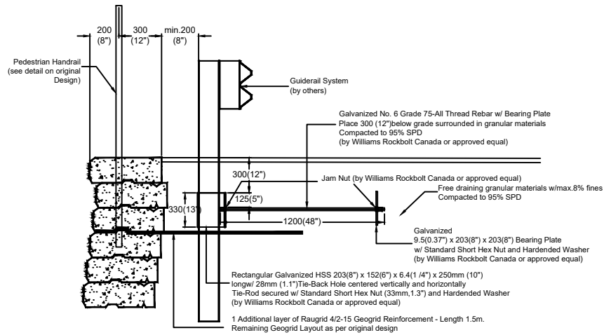
SECTION VIEW
