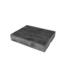
COPING 400mm x 75mm x 325mm 15 3/4" x 3" x 12 7/8"
