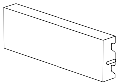
6" STANDARD FASCIA PANEL 150 x 466 x 60mm 5 7/8 x 18 3/8 x 2 3/8" 84 Units/Bundle .73 Sq.Ft./Stone
